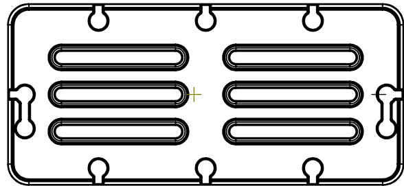
5948I 48 X 22 X 12 in 122 X 56 X 30 cm
